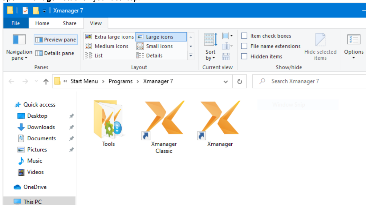
Fig. 1: Xmanager Folder
