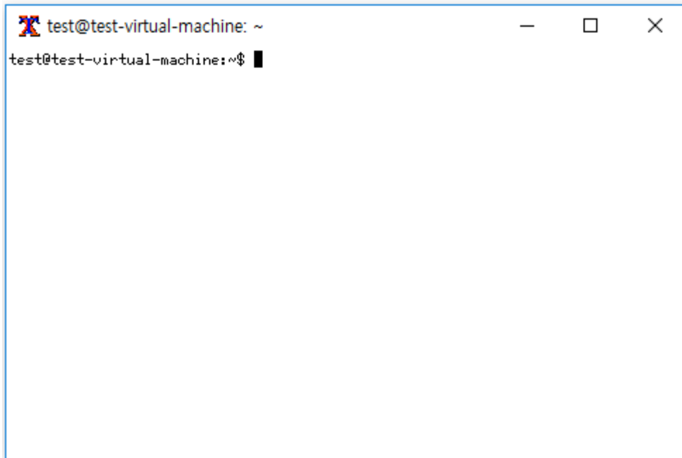
Fig. 8: xterm window
